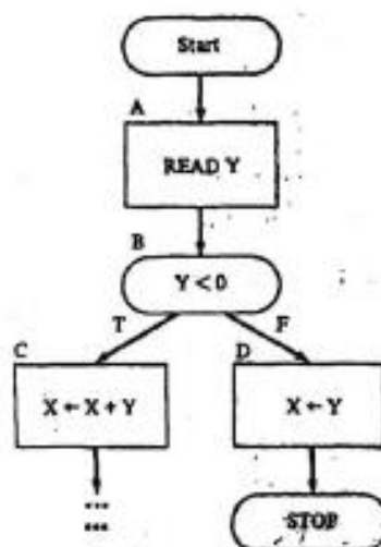
Figure 5.1 A code segment and control flow graph
