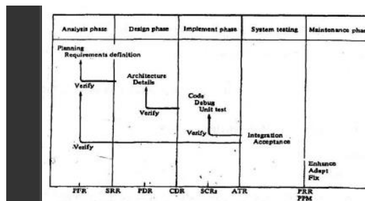
Figure 2.3 Reviews and milestones in the phased life-cycle model
