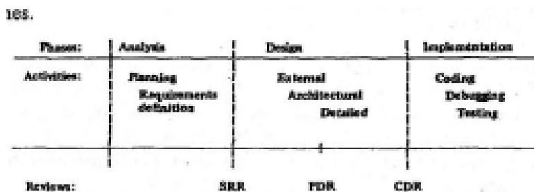
Figure 4.1 Tuning of the Software Requirements Review (SRR), the Preliminary Design Review (PDR), and the Critical Design Review (CDR).
