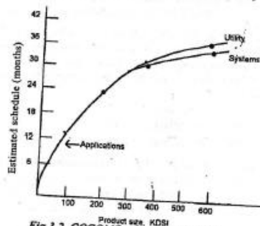
Fig.3.2 COCOMO schedule estimates
